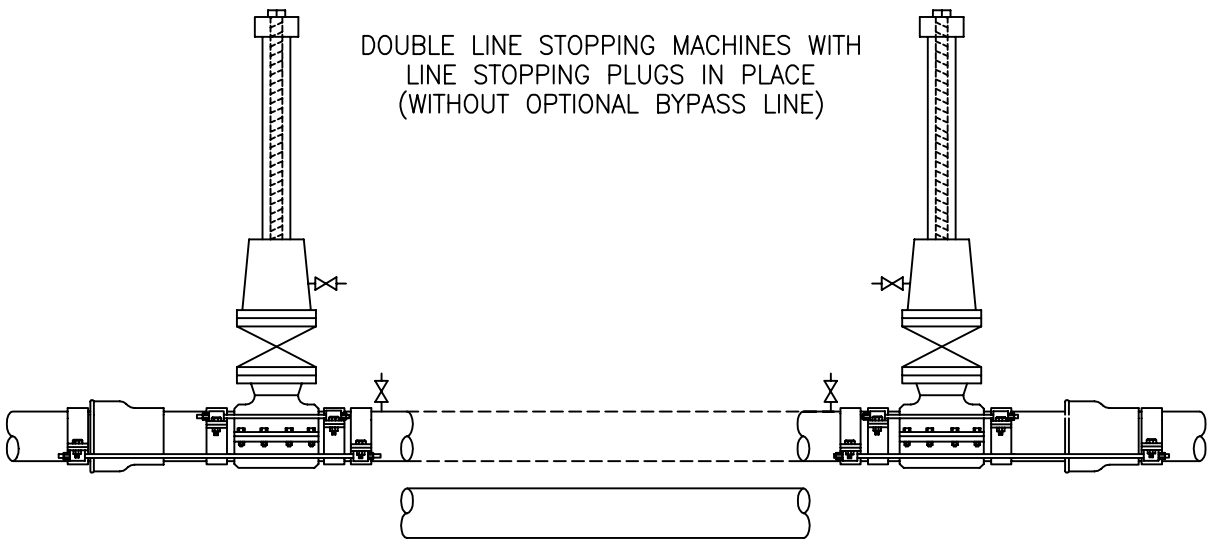
DOUBLE LINE STOPPING MACHINES WITH LINE STOPPING PLUGS IN PLACE (WITH OPTIONAL BYPASS LINE)
